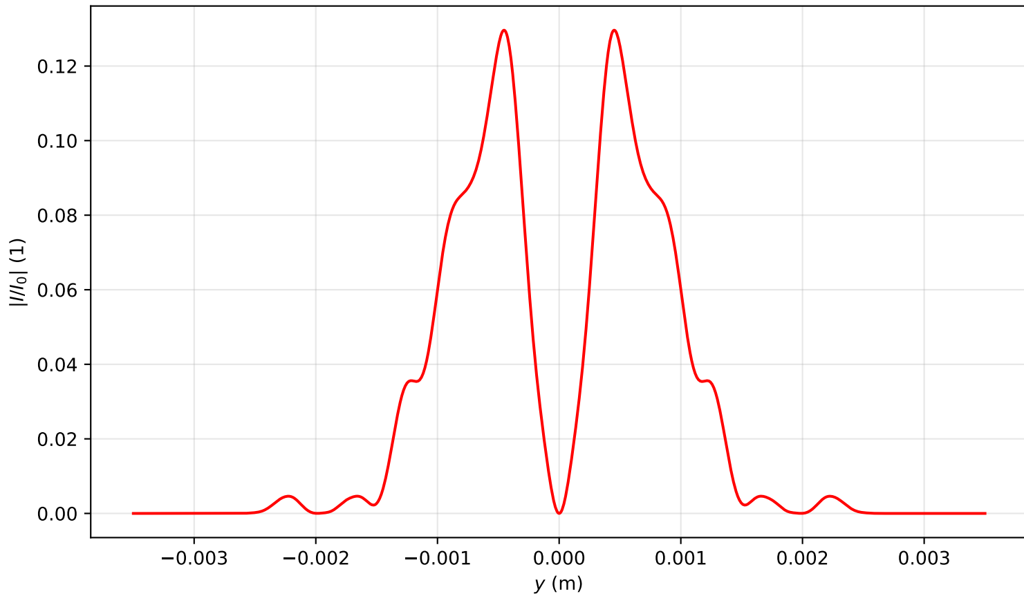
Intensity profile I(x=0, y, z=3.025)/I_0 , P_{in}=7.0P_{cr} , artificial time
